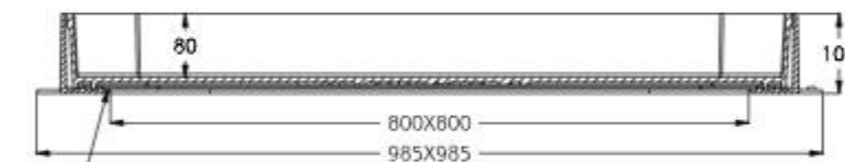
GRP PROVISION SECTION A-A
