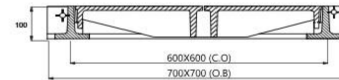
SECTION VIEW
