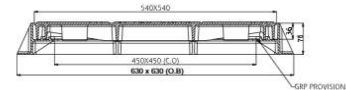
FRONT VIEW SECTION "A - A"
