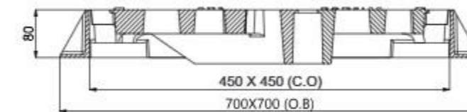
SECTION VIEW
